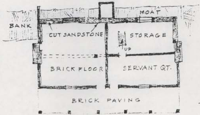
BASEMENT PLAN
