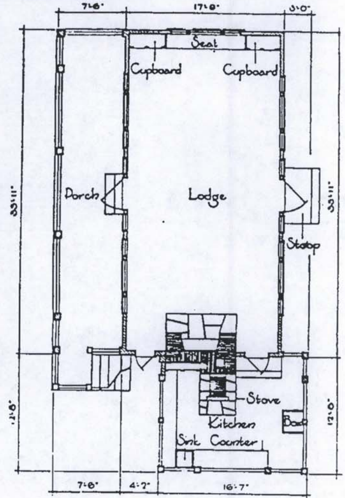
ILLUSTRATION 1: PLANS FOR CAMP (2) MAWAVI (from Park and Recreation Structures , Good)
