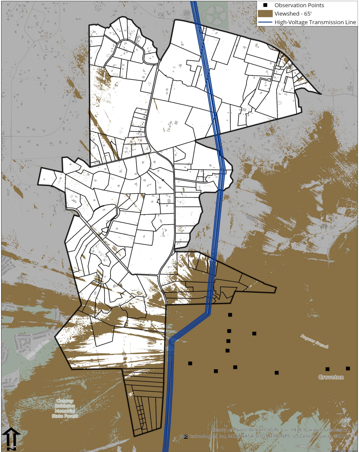
Figure 9: 65' Viewshed Analysis
