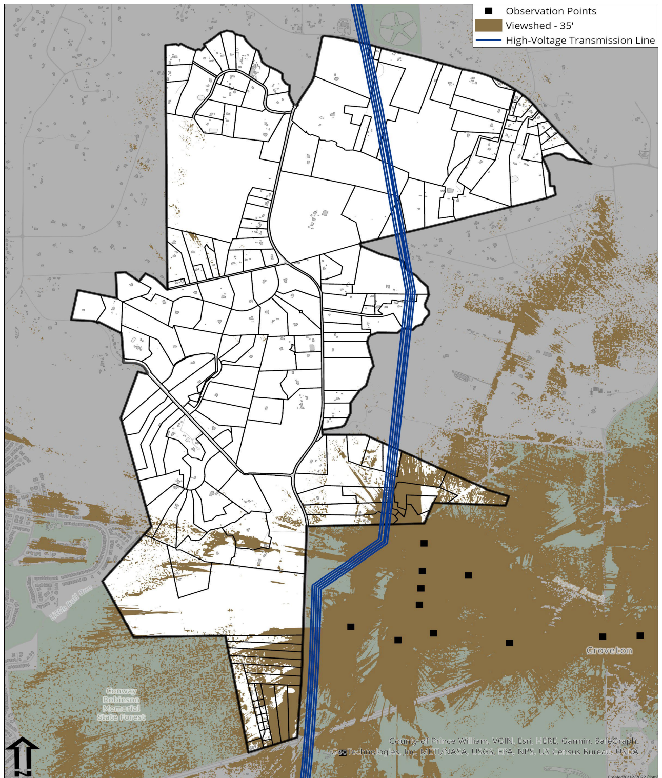
Figure 7: 35' Viewshed Analysis
