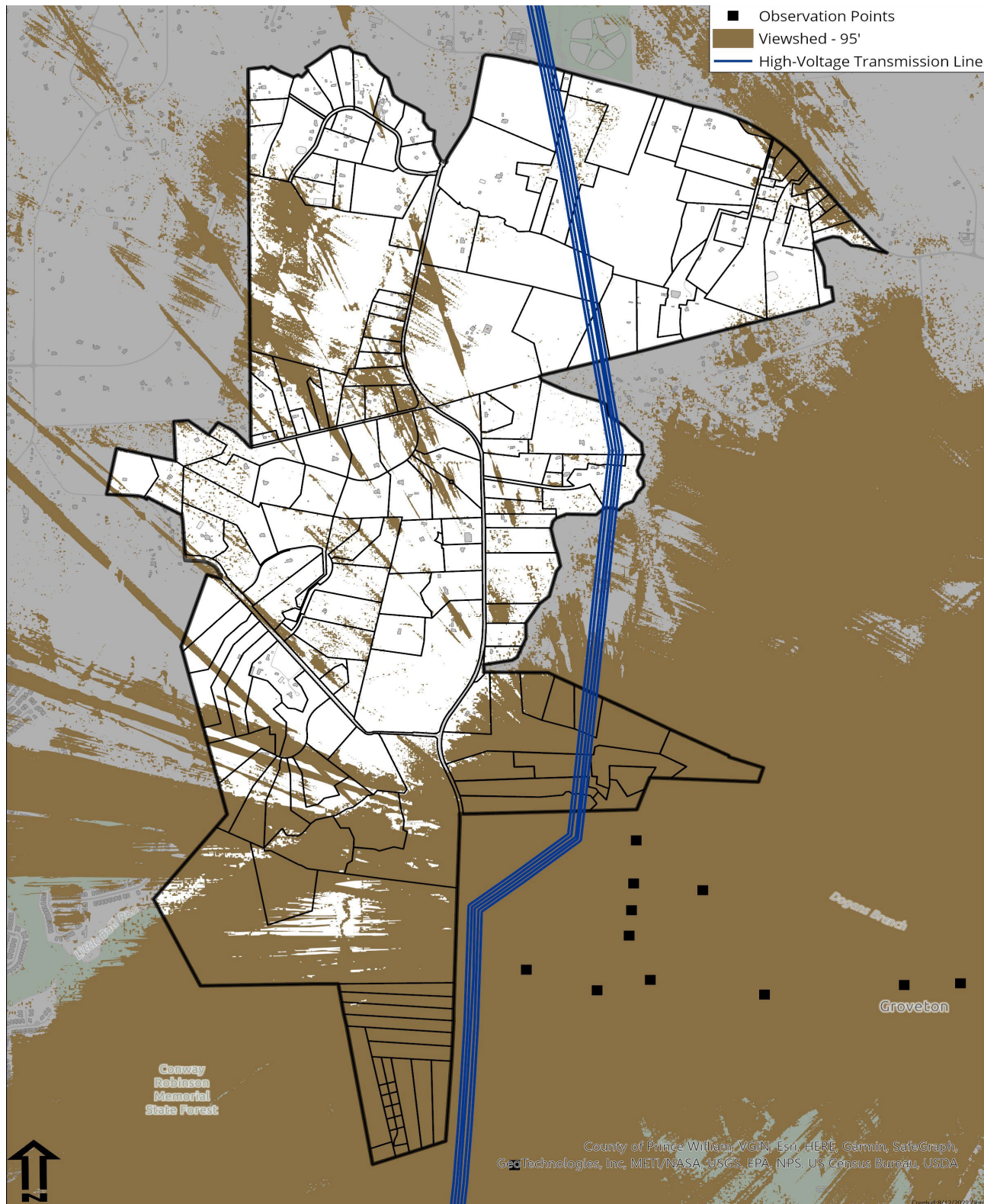
Figure 11: 95' Viewshed Analysis
