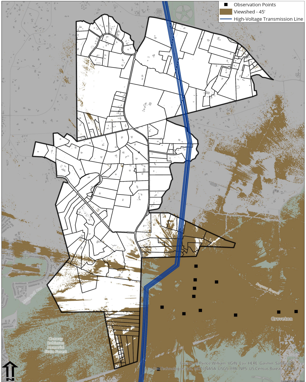
Figure 8: 45' Viewshed Analysis
